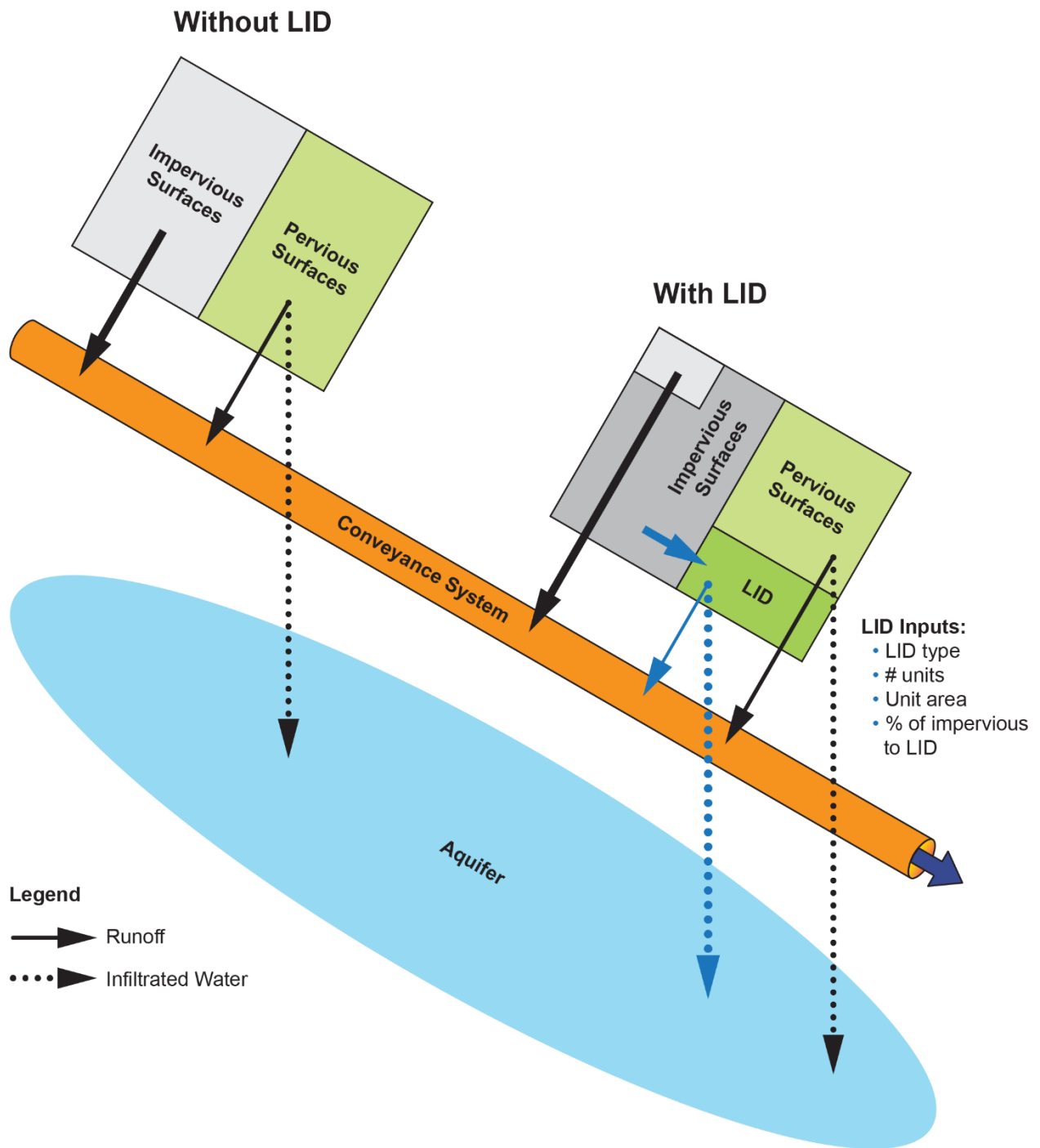
FIGURE 11-1. CONCEPTUAL REPRESENTATION OF GSI MODELING IN SWMM5
