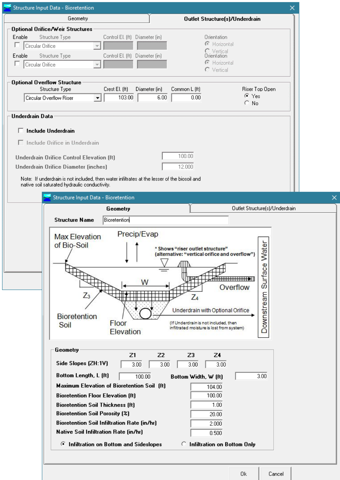
FIGURE 12-3 BIORETENTION FACILITY DEFINITION WINDOW
